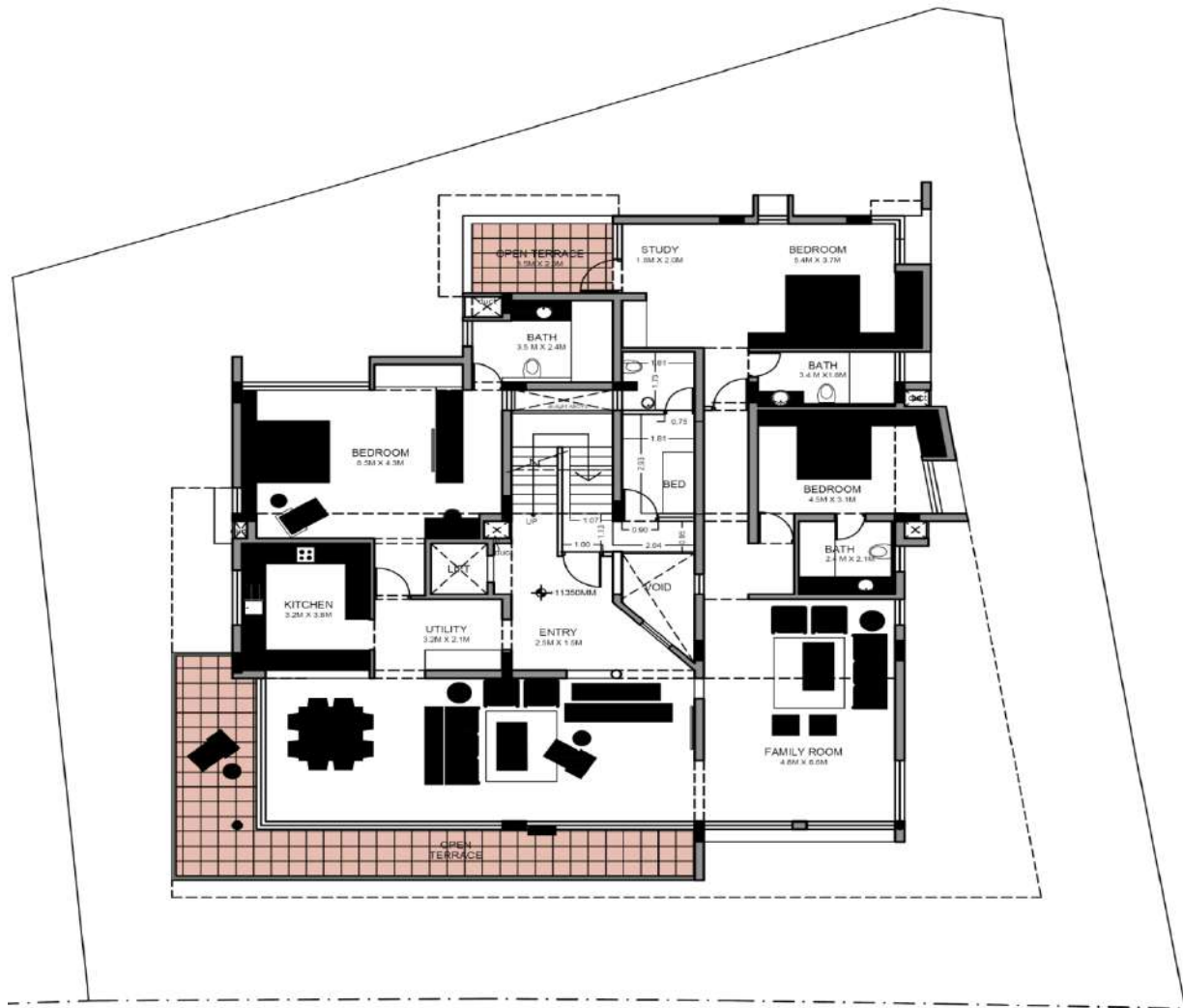
THIRD FLOOR @ +11.65M
